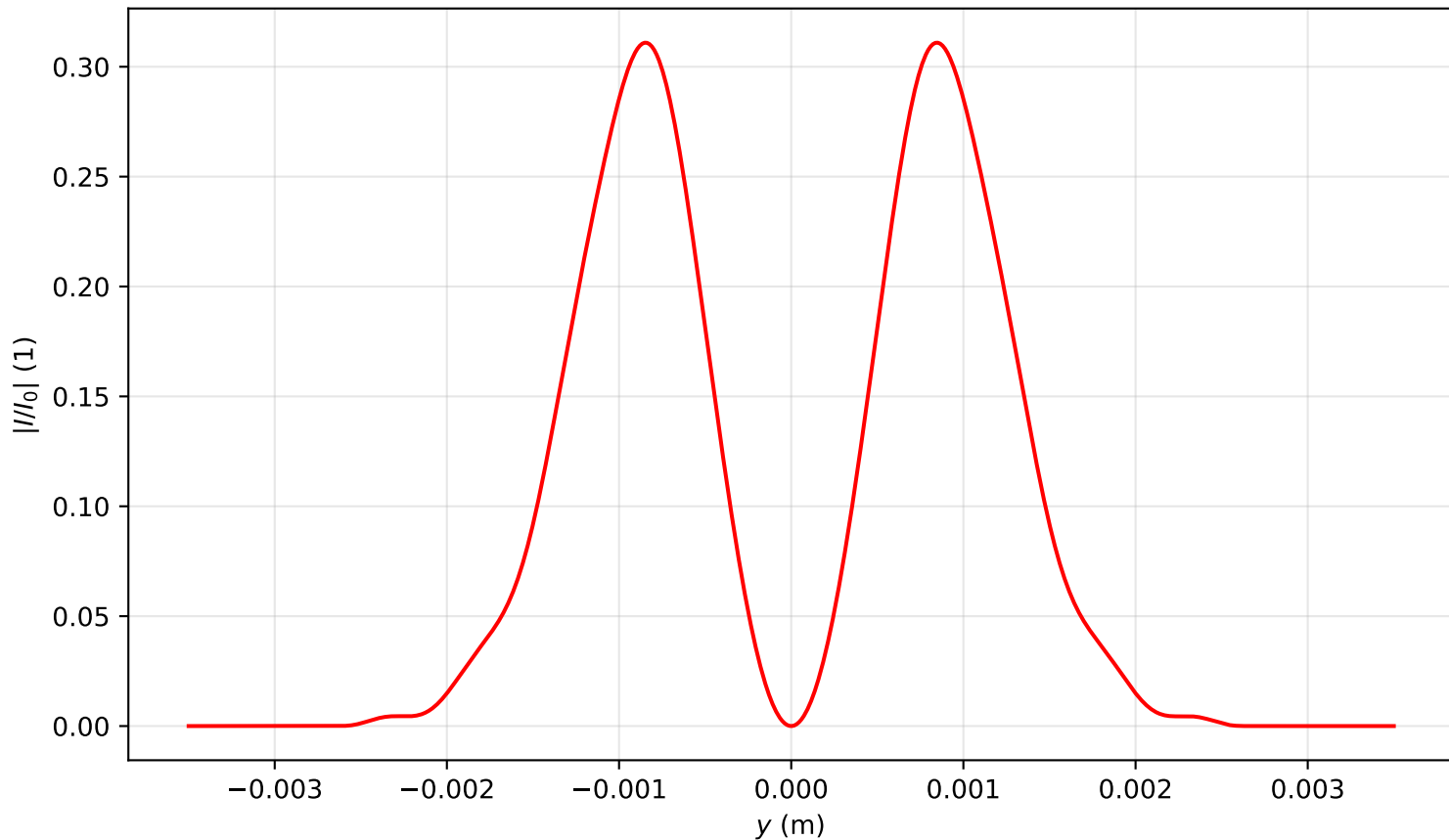
Intensity profile I(x = 0, y, z = 3.264)/I_0 , \text{Pin}=2.0\text{Pcr} , artificial time
